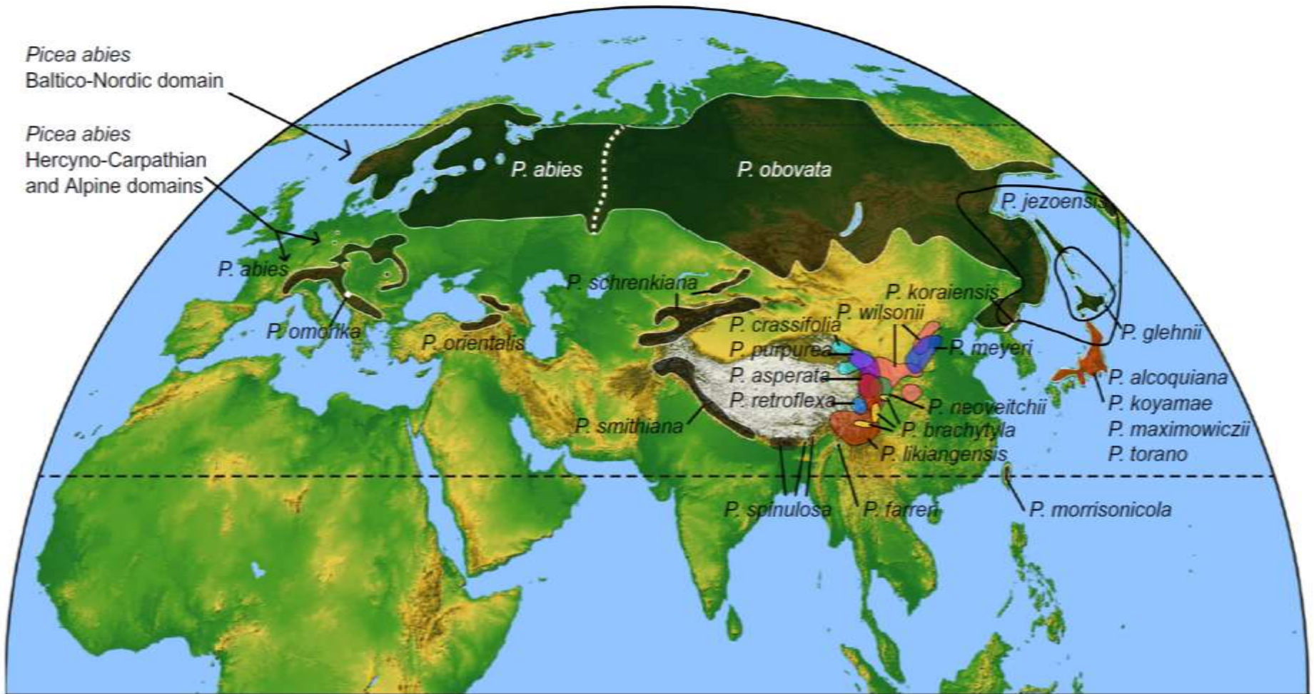
1. Map of the Northern Hemisphere in equal-area projection (Mollweide) showing the distribution of Picea based on Farjón (1990) and eFloras (2008). Black dashed line indicates the equator. From Lockwood, J.D. et Al - (2013) - A new phylogeny for the genus Picea , in Molecular Phylogenetics and Evolution 2013, Vol.69/3, p. 717-727
